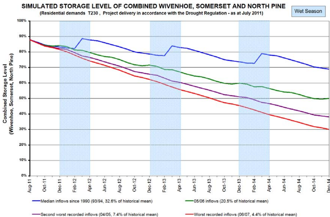
Figure 1: Forecast Wivenhoe, Somerset and North Pine Dam storage levels based on repeated inflows
