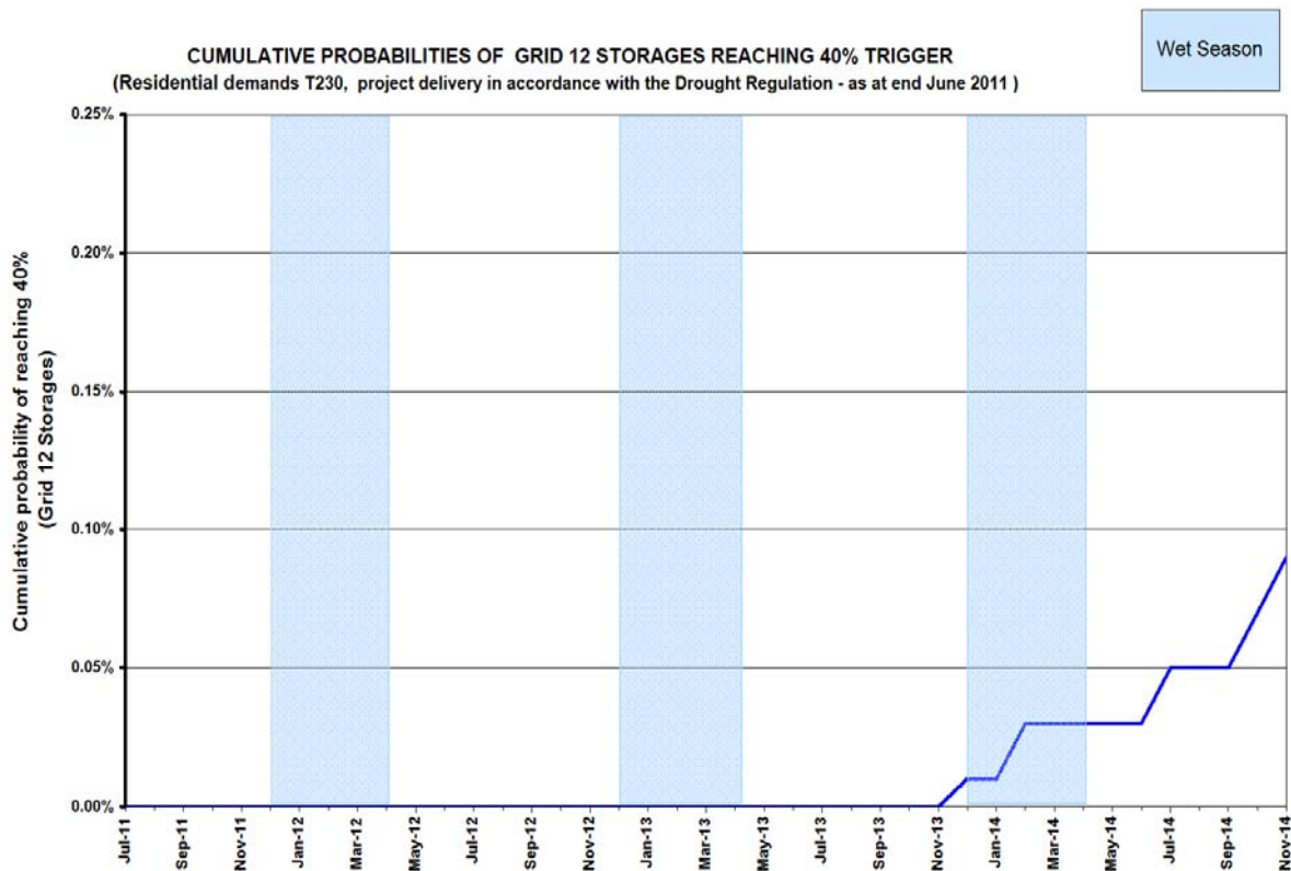
Figure 2: Forecast cumulative probability of Grid 12 storages reaching 40%
