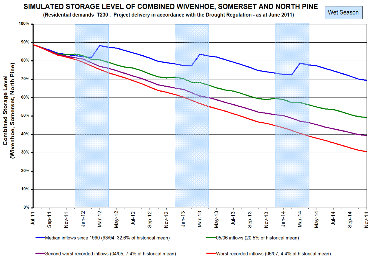
Figure 1: Forecast Wivenhoe, Somerset and North Pine Dam storage levels based on repeated inflows
