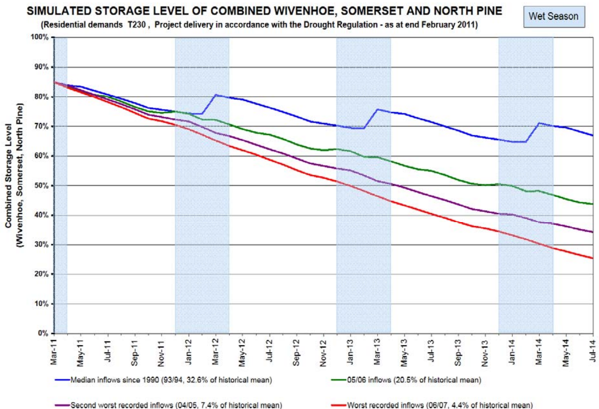
Figure 1: Forecast Wivenhoe, Somerset and North Pine Dam storage levels based on repeated
