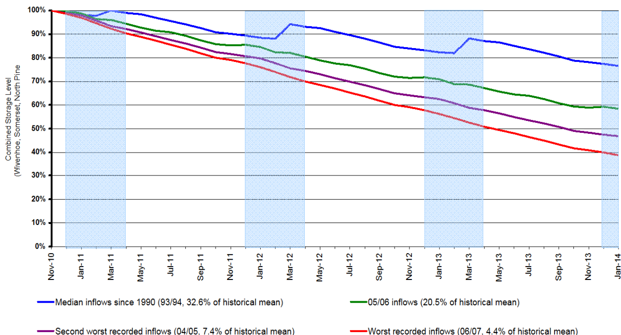
Figure 1: Forecast Wivenhoe, Somerset and North Pine Dam storage levels based on repeated inflows
